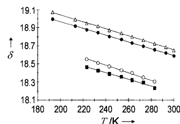
Figure 2. Temperature dependence of the hydrogen-bridge hydron chemical shift for the isotopomers of 1 . ^1\text{H} for HH ( \Delta ), ^1\text{H} for HD ( \bullet ), ^2\text{H} for HD ( \circ ), and ^2\text{H} for DD ( \blacksquare ).
